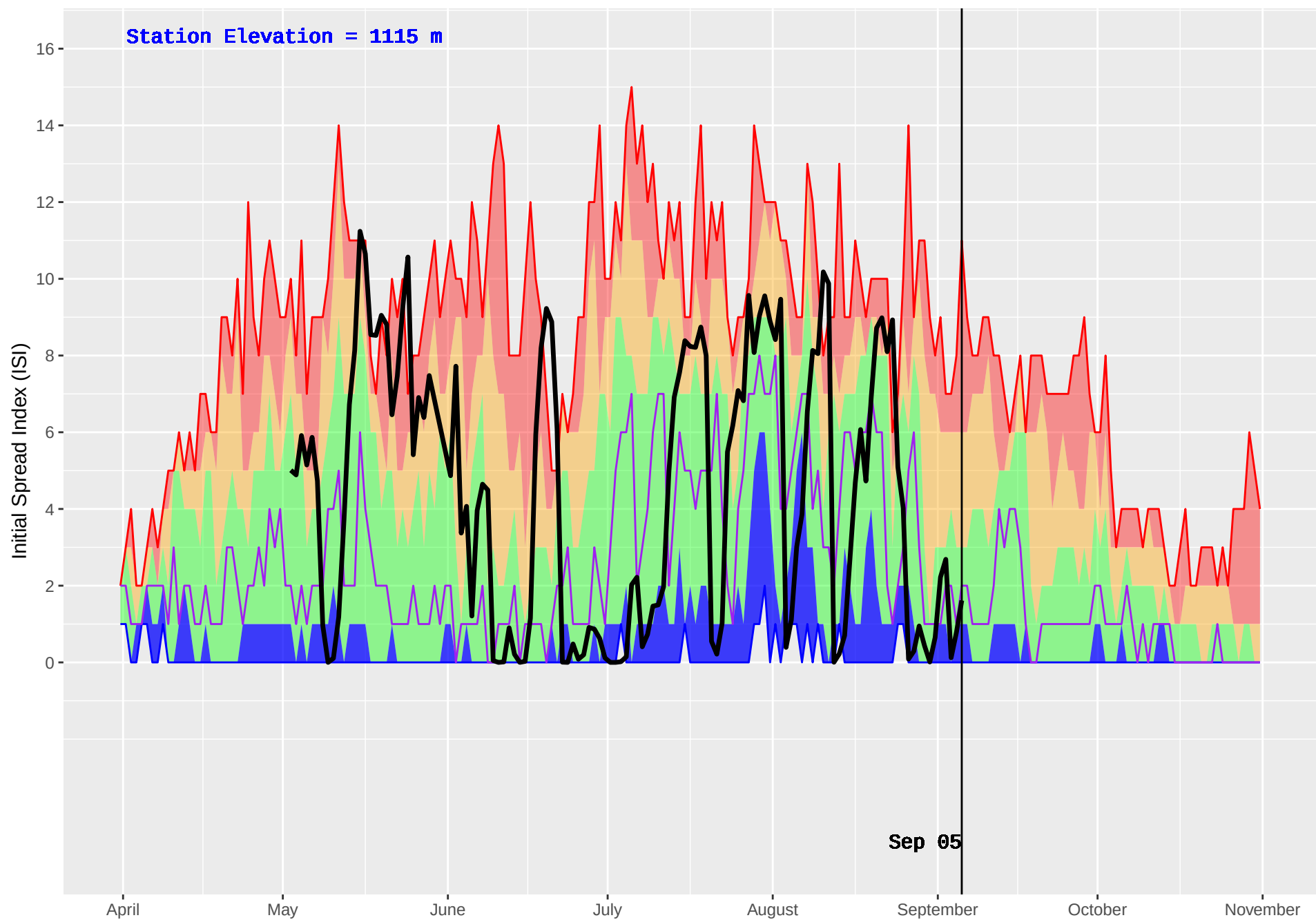
SICAMOUS (882) : Historical (2004–2016) and Current (2018) Daily Initial Spread Index (ISI)
