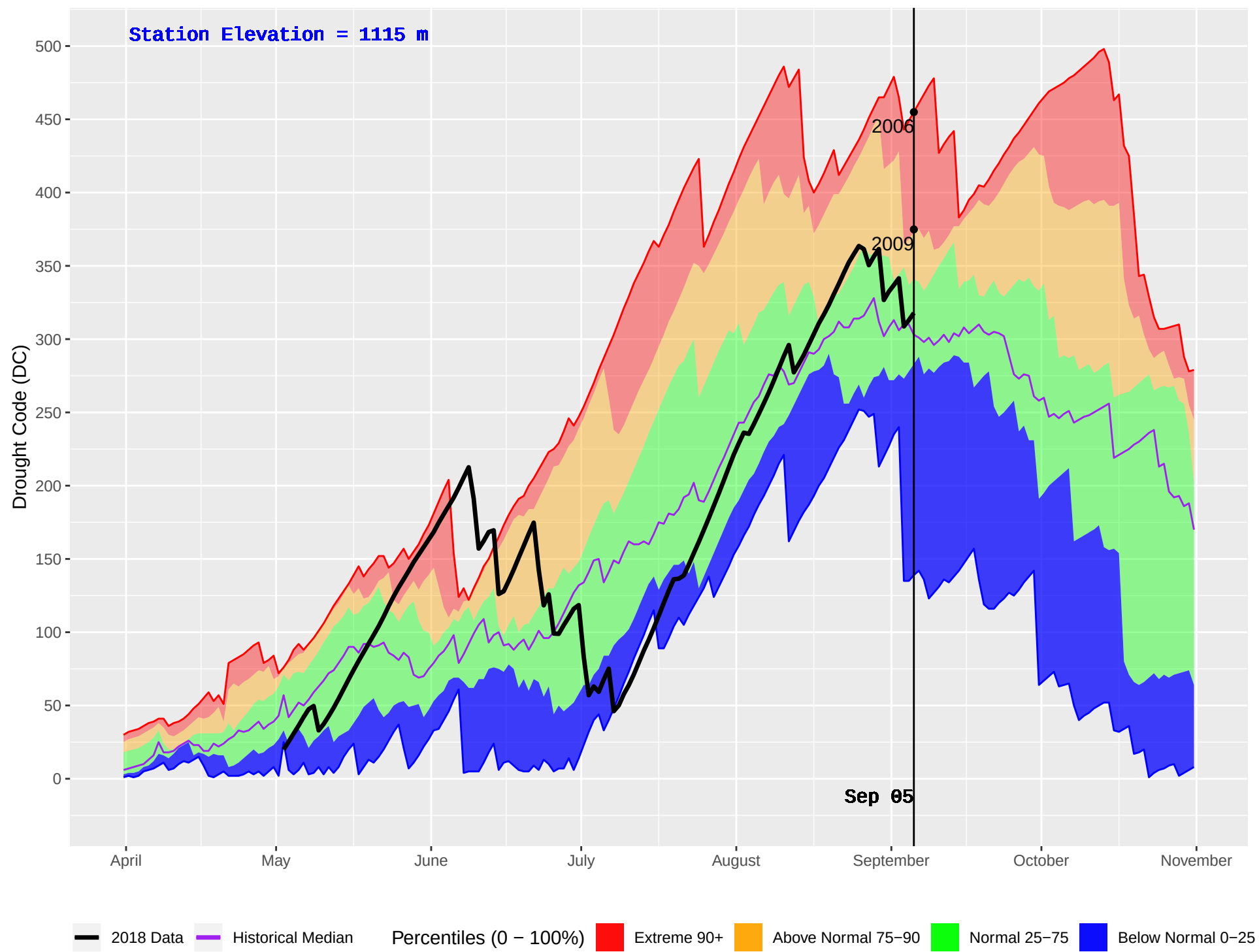
SICAMOUS (882) : Historical (2004–2016) and Current (2018) Daily Drought Code (DC)
