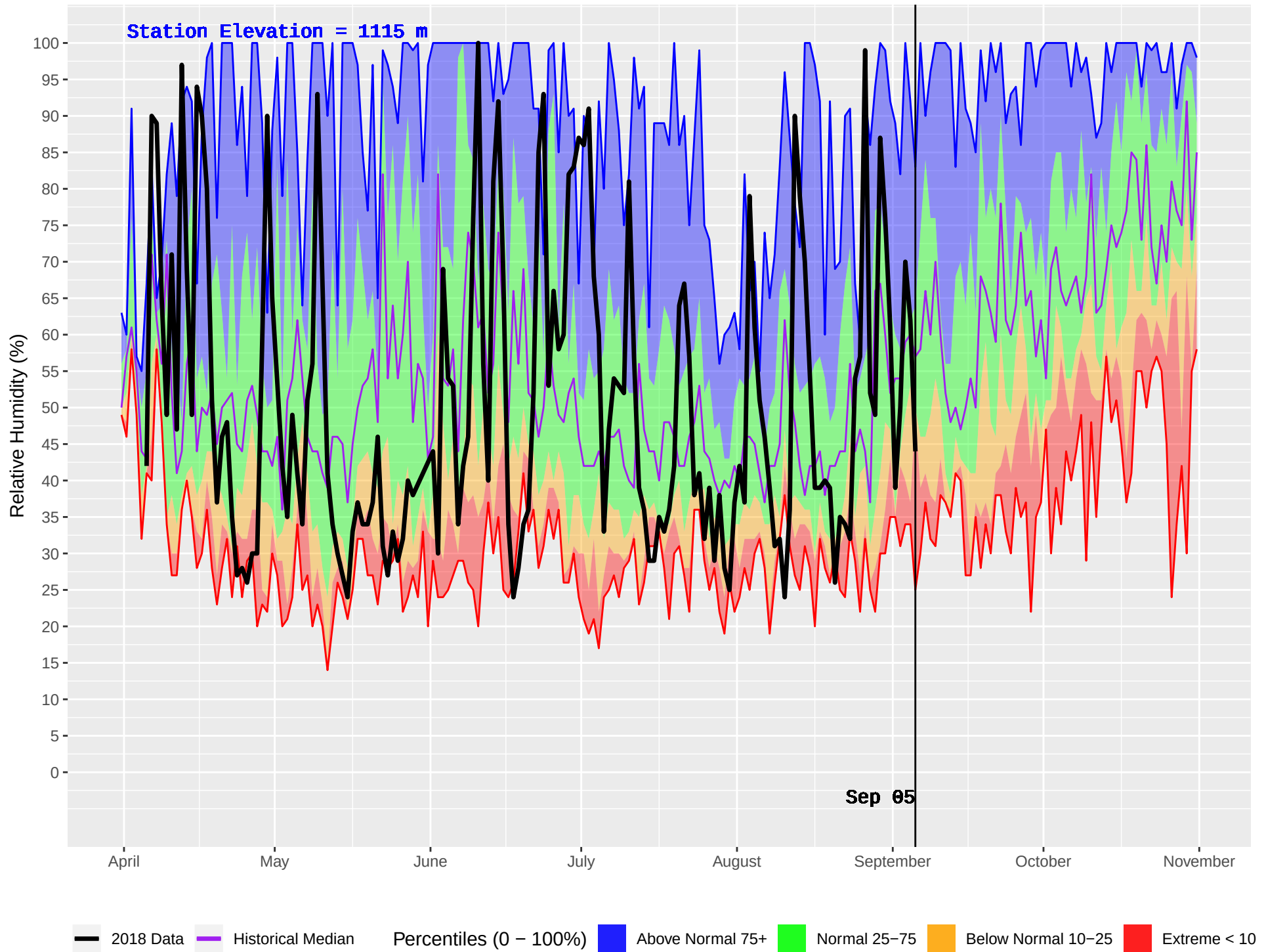
SICAMOUS (882) : Historical (2004–2016) and Current (2018) Daily Relative Humidity
