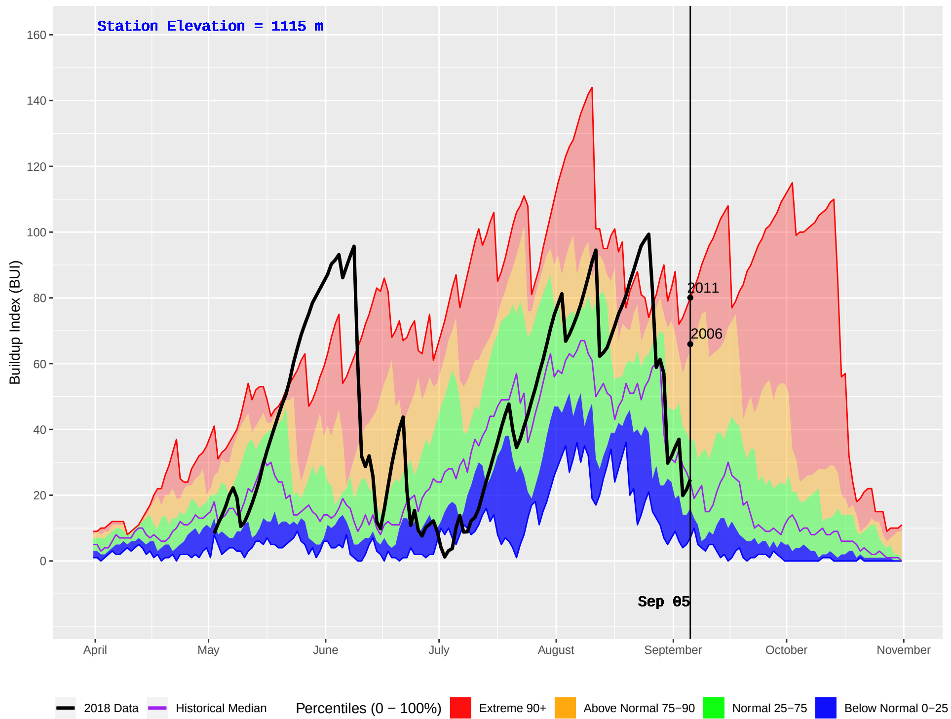
SICAMOUS (882) : Historical (2004–2016) and Current (2018) Daily Buildup Index (BUI)
