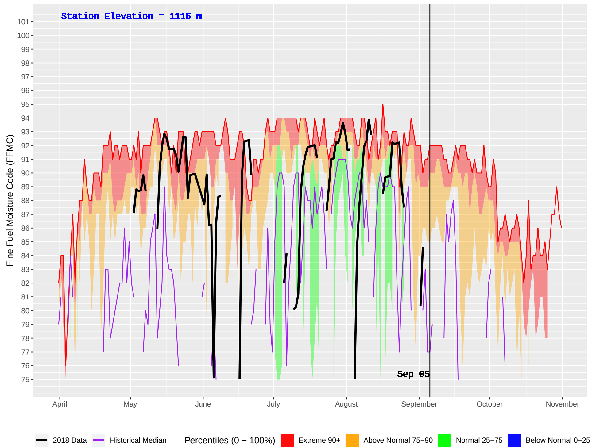
SICAMOUS (882) : Historical (2004–2016) and Current (2018) Daily Fine Fuel Moisture Code (FFMC)
